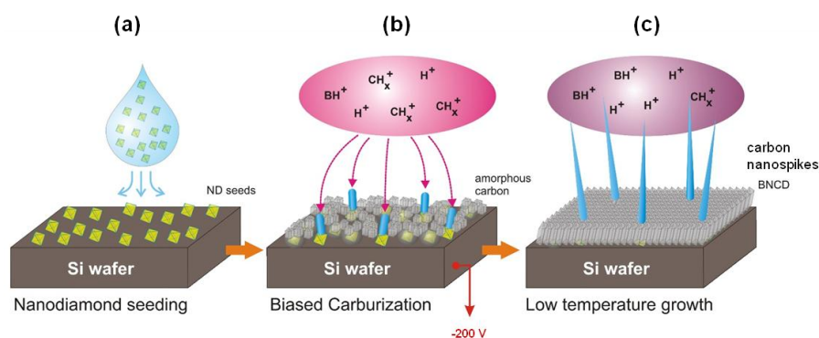
42 Figure 8. Scheme of the growth mechanism of BNCD-CNS hybrids in the H_2/CH_4/B_2H_6/N_2 43 microwave plasma-(a) the nanodiamond seeding on the Si wafer prior to diamond growth, (b) 44 and (c) the sub-sequential steps of nanospike formation of BNCD-CNS hybrids in the microwave 45 plasma. 46 47 48 49
