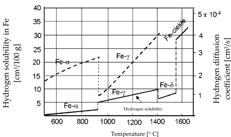
Fig. 2. Solubility of hydrogen in iron depending on temperature and pressure [20]
