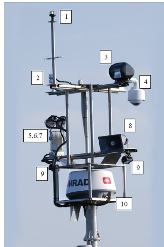
Fig. 4. Devices on the platform mast: 1) top lamp, 2) weather station, 3) searchlight – controlled head, 4) fisheye camera – platform supervision, 5) thermal imaging camera, 6) camera of visible light, 7) positioning system of thermal imaging camera and visible light, 8) megaphone for generating messages, 9) work lighting – LED, 10) radar
