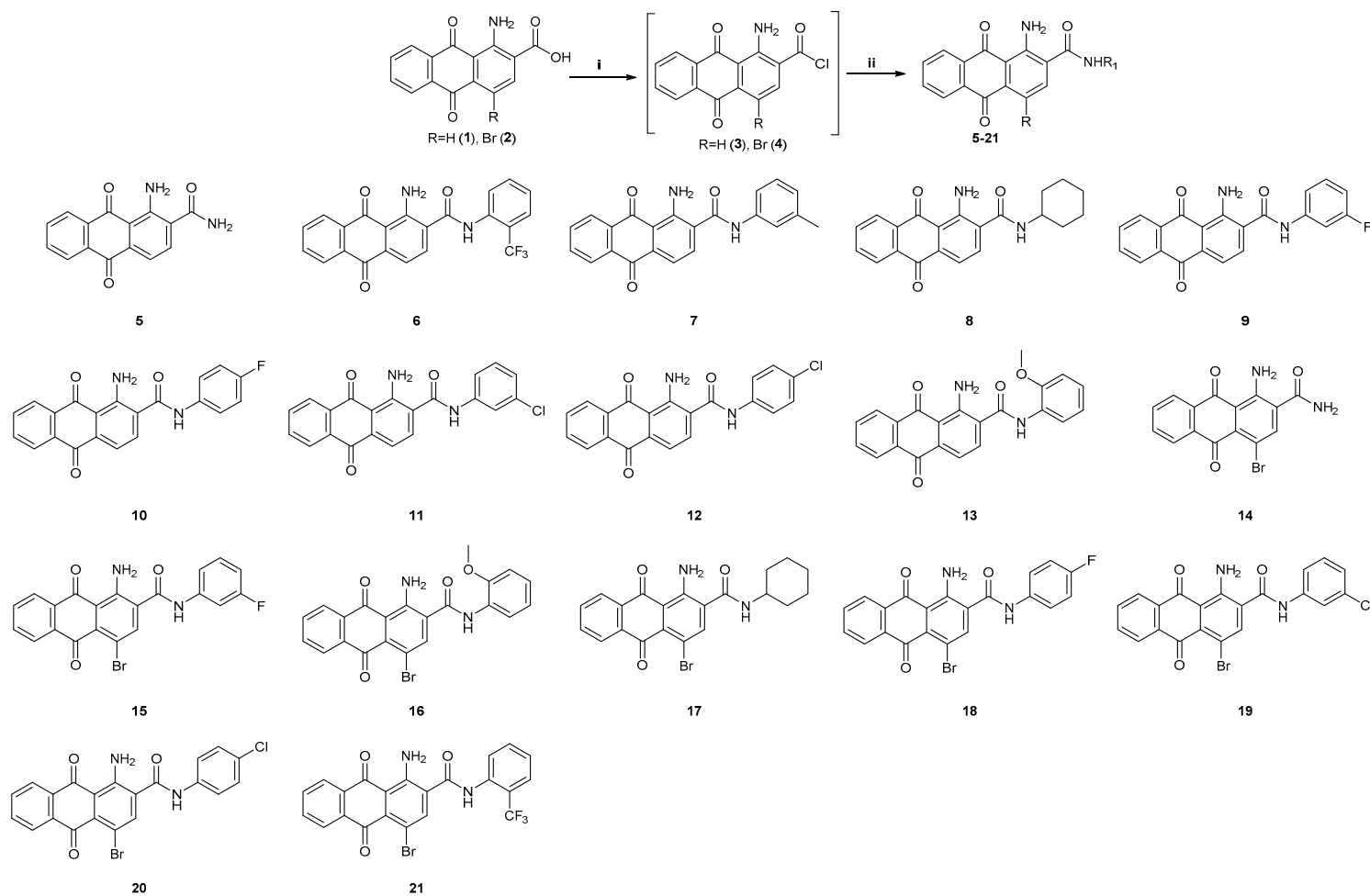
Scheme 1. Synthesis of amides 5–21. Reagents and conditions: (i) thionyl chloride (3 equiv), pyridine (0.15 equiv), dry benzene, 80 °C, 5 h, (ii) for compounds 5 and 14—25% NH 4 OH (50 mL), -15 °C, 1 h → 80 °C, 3 h → r.t., 10% HCl; for compounds 6–13, 15–21—R 1 NH 2 (1.1 equiv), dry benzene, TEA (1.1 equiv), Δ, 12 h.
