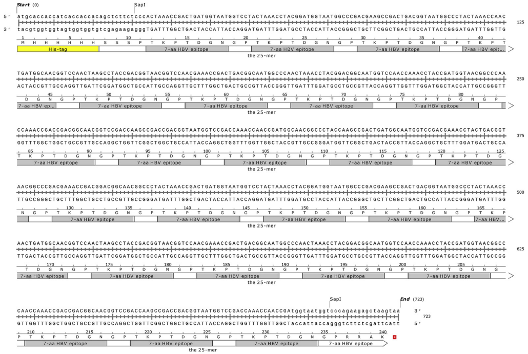
Fig. 5. DNA and aa sequences of the designed 25-mer of the 7-aa HBV epitope. The DNA gene sequence was optimized for expression in E. coli . The gene was chemically synthesized, cloned into the Sapl-cleaved pAMP1-HisA vector and subjected to the amplification process.
