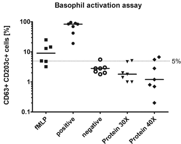
Fig. 11. In vitro activation of basophils in the presence of activating antibodies (first positive control), fMLP (second positive control), the AGF_30 protein, the AGF_40 protein (1 \mu g/ml) and negative control. Results are presented as a single data (% of activated basophils for each patient) and median.
