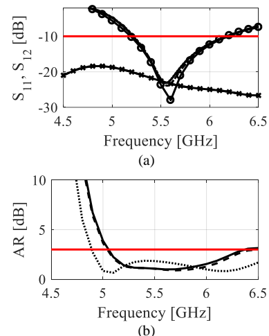
FIGURE 11. Bending effects on the antenna characteristics (a) |S_{11}| , r = 0\text{ mm} bend (o—o), r = 15\text{ mm} bend (—), and r = 35\text{ mm} bend (---), and |S_{12}| , r = 15\text{ mm} bend (—), and r = 35\text{ mm} bend (-x-), (b) AR, r = 0\text{ mm} bend (....), r = 15\text{ mm} bend (—), and r = 35\text{ mm} bend (---).
