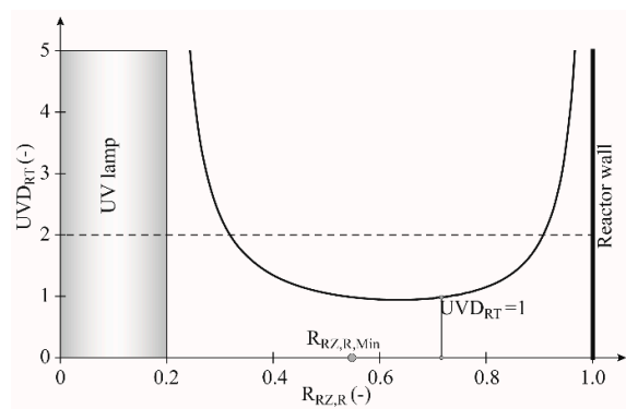
Figure 7. The relation between the UV radiation dose and the integral radius in the radiation zone.
