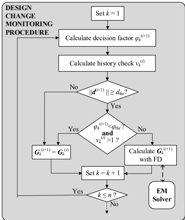
Fig. 2. Flow diagram of design change monitoring procedure (DCMP). The following notation is used: G_k^{(i)}(f) – the k -th column of the antenna response gradient \mathbf{G}_s ; \|d^{(i)}\| – the size of TR region; d_{\text{thr}} – user-specified trust-region size threshold; \varphi_k^{(i)} – the decision factor; \varphi_{\text{thr}} – user-specified threshold for decision factors; v_k^{(i)} – update history count; the indices k and i refer to the parameter and algorithm iteration number, respectively.
