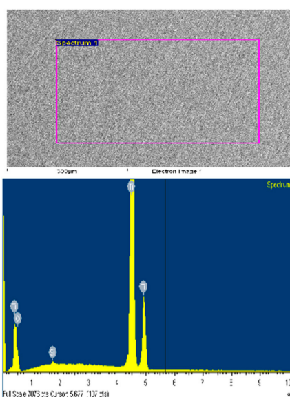
Figure 2. Surface chemical composition after gas oxidation of titanium.
