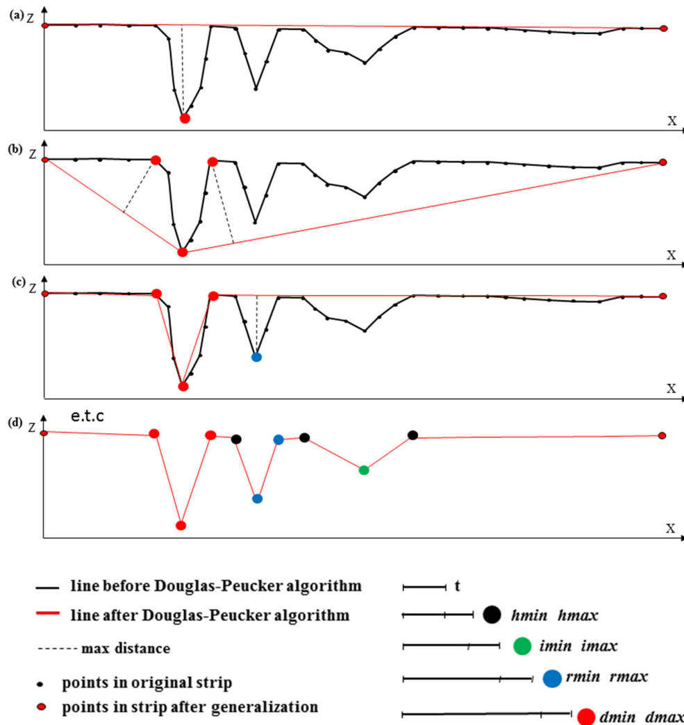
Figure 2. Modification of the Douglas-Peucker algorithm.
