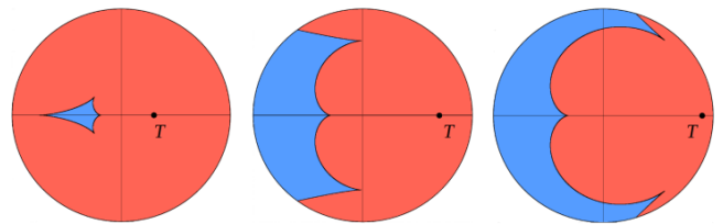
FIGURE 3. Catacaustic regions for 1 st order reflections.
