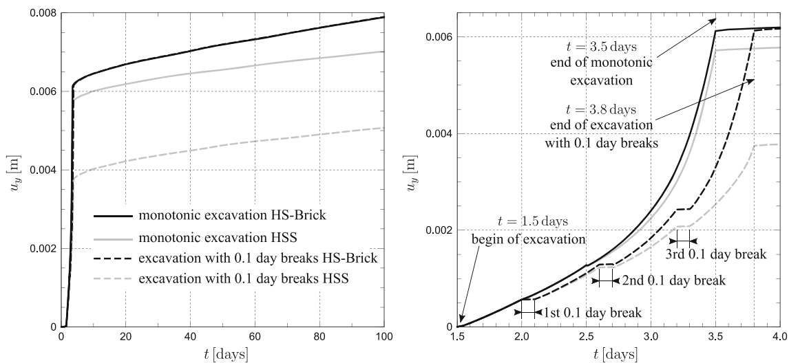
Fig. 11 Calculated vertical heave of the point located in the middle of the excavation bottom. Left: heave during excavation and consolidation up to t = 100 days. Right: magnification of the heave changes during the excavation simulation with two applied time sequences. In the case of the HS-Brick model, the small consolidation breaks only shift the parts of heave–time curve, whereas in calculations with the HSS model additionally inclination changes of the heave–time curve are observed, leading to smaller deformation when compared with monotonic excavation
