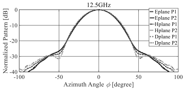
Fig. 7. The radiation pattern for two polarizations in E-plane ( \varphi=90 ), H-plane ( \varphi=0 ) and D-plane( \varphi=45 ).
