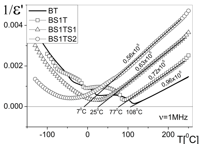
Fig. 8. The inverse of the real part of dielectric permittivity ( 1/\varepsilon' ) as a function of temperature for BT, BS1T, BS1TS1 and BS1TS2 samples at chosen frequency 1 MHz
