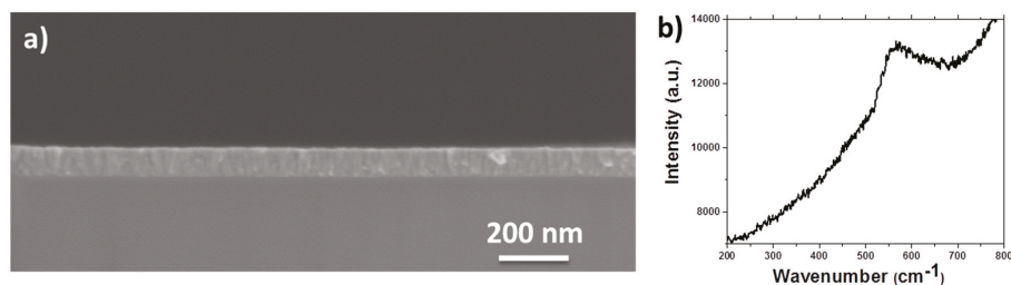
Figure 4. (a) SEM cross section image of TiO 2 films deposited by ALD on Si substrates and (b) Raman spectrum of TiO 2 films deposited by ALD.
