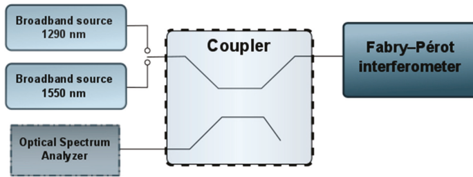
Figure 5. Design of the experimental sensor.
