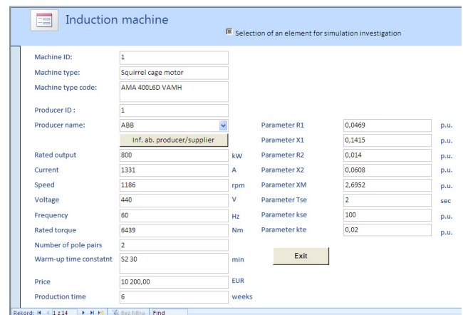
FIGURE 5. Catalogue card with data of chosen motor from component's base of ship thruster structures, prepared in MS Access application.
