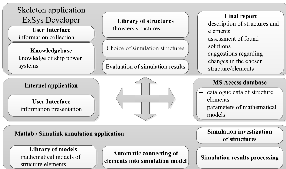
FIGURE 1. Elements of hybrid expert system supporting design of ship’s power subsystems.
