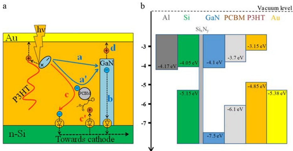
Fig. 8 a Mechanism explaining electric current generation processes in BHI/GaN NWs/Si cascade junction. Following photo-current components are contributed by respective interfaces: a P3HT/GaN NW interface and a' by P3HT:PCBM blend. b electron
