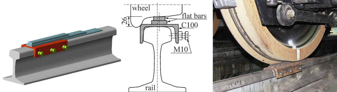
Fig. 3. Steel wedge for impulse excitation of the car.
