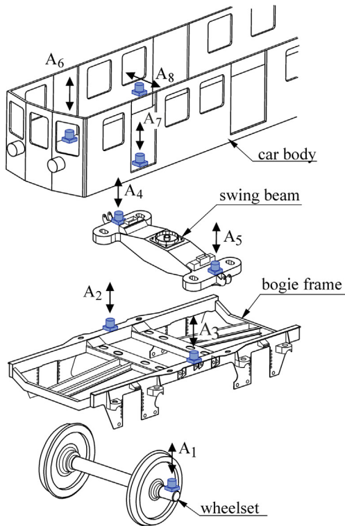
Fig. 4. Measuring sensor locations.
