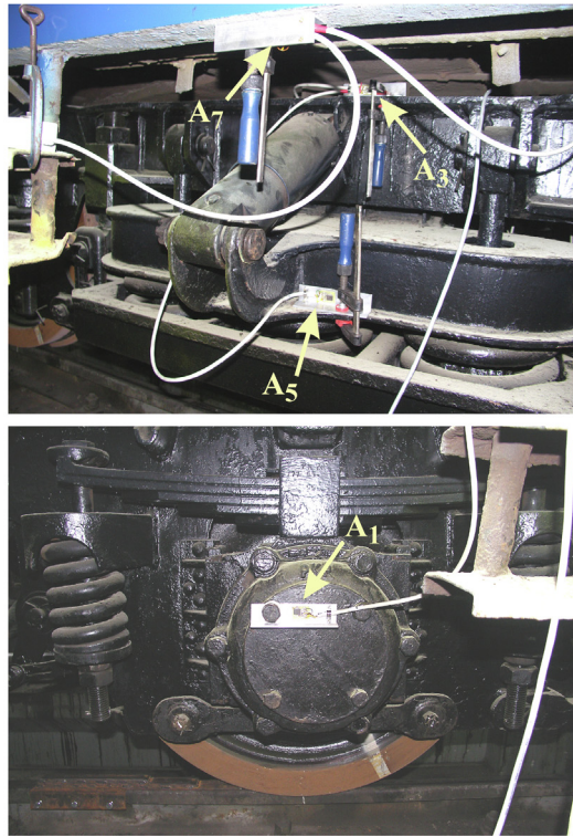
Fig. 4. Measuring sensor locations.
