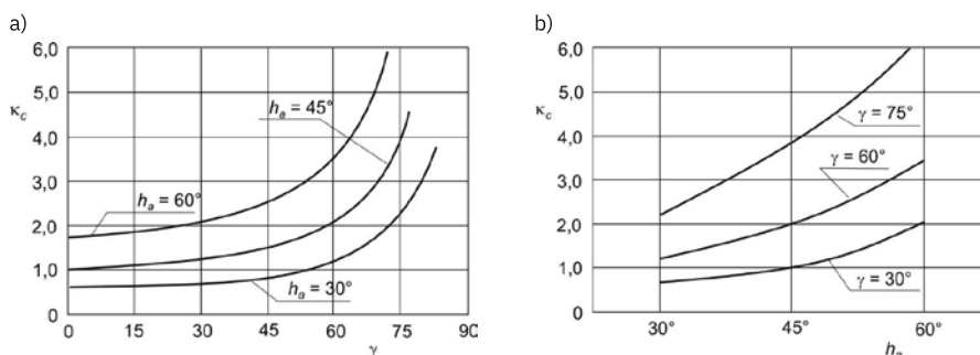
Fig. 2a. The value of the facade shading measured from the overhanging elements, with respect to the location of the building relative to the four compass points (angle h_a ), assuming different values of solar angular height h_a
