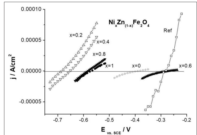
FIGURE 14 | Linear polarization plots for carbon steel in nano-ferrite and nano- \text{Fe}_2\text{O}_3 extracts.
