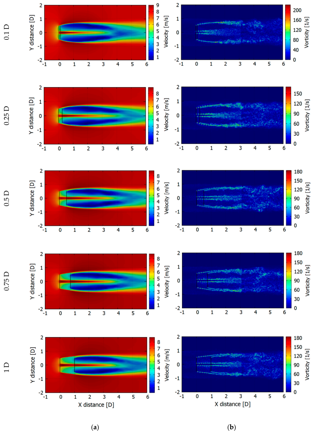
Figure 13. Mean velocity (a) and vortices (b) contours for CRWT operating with TSR_1 = TSR_2 = 5 .
