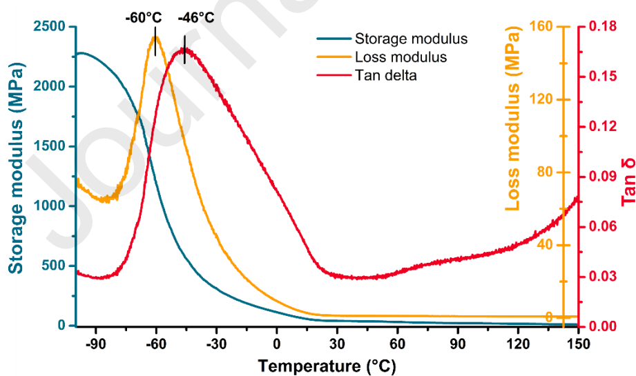
Figure 4 DMA curves of Bioflex® printout - storage, loss modulus and damping parameter.
