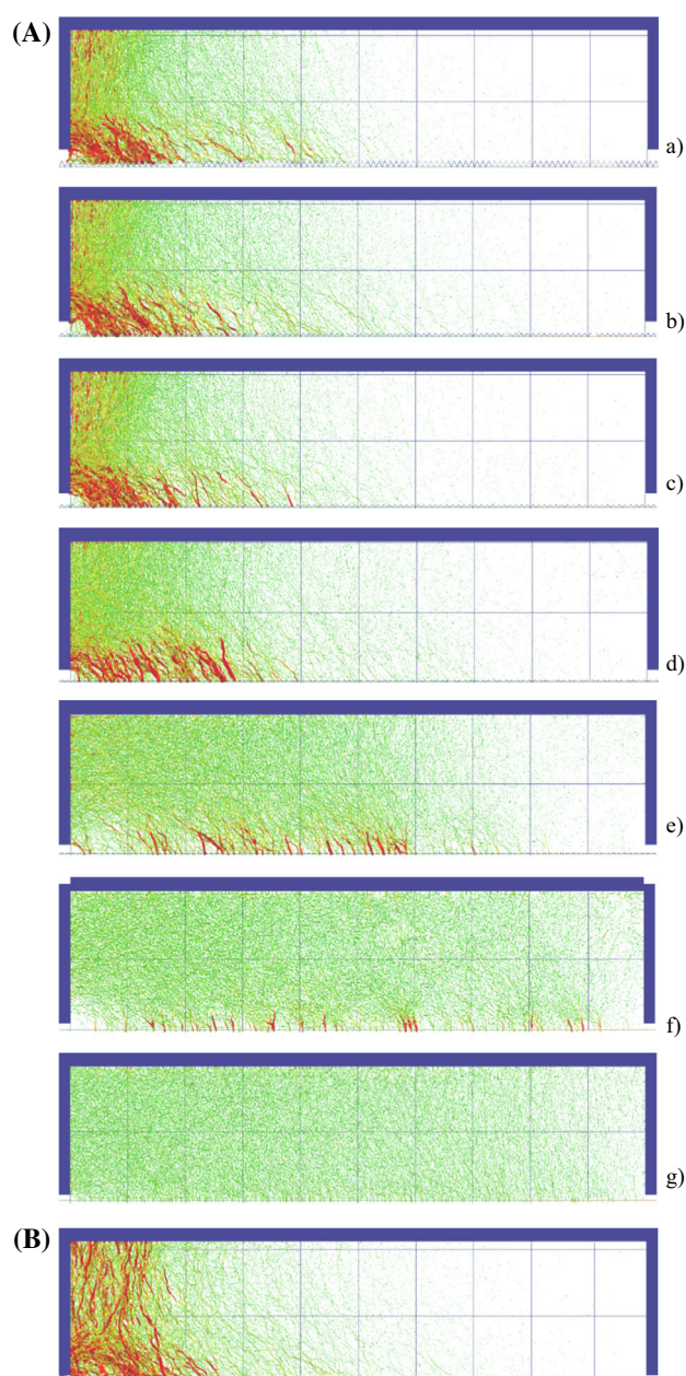
Fig. 17 Distribution of contact normal forces in granular specimen at residual state for u_x = 7.0 mm from DEM with: A ) different normalized roughness parameter ( e_o = 0.55 and \sigma_n = 100 kPa): a R_n = 2.0 , b R_n = 1.0 , c R_n = 0.75 , d R_n = 0.50 , e R_n = 0.25 , f R_n = 0.10 and g R_n = 0.01 and B ) different initial void ratio ( e_o = 0.80 , \sigma_n = 100 kPa and R_n = 1.0 ) (red colour corresponds to normal contact forces higher than mean value, maximum value of forces is 0.50 N)
