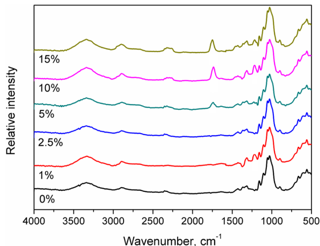
Fig. 7 FTIR spectra of UFC100 fillers modified with varying content of IPDI
