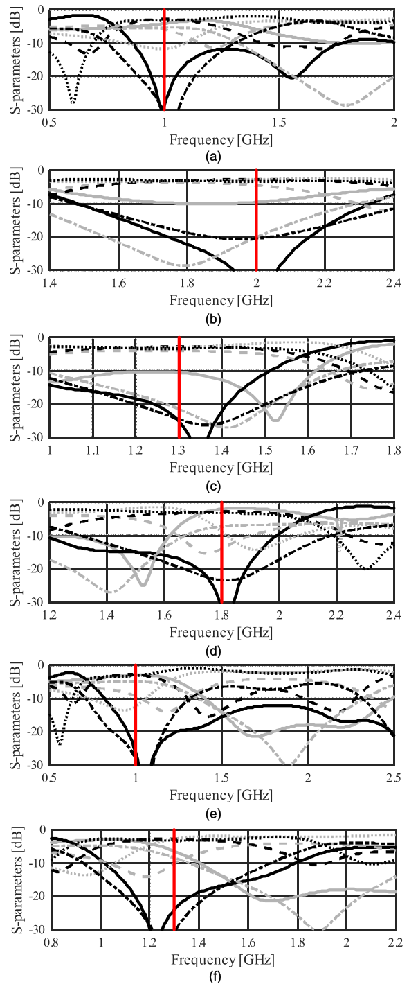
FIGURE 5. Optimized designs of miniaturized rat-race coupler Fig. 3 obtained using the proposed regularization scheme (black) starting from the initial designs of Table 1 (gray) for different values of the target operating frequencies: (a) f_0 = 1.0 GHz, (b) f_0 = 2.0 GHz, (c) f_0 = 1.3 GHz, (d) f_0 = 1.8 GHz, (e) f_0 = 1.0 GHz, and (f) f_0 = 1.3 GHz. Shown are the S-parameters of RRC: S_{11} (—), S_{21} (---), S_{31} (···), and S_{41} (-).
