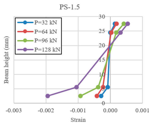
Figure 16. Strain diagram for beam PS-1.5.
