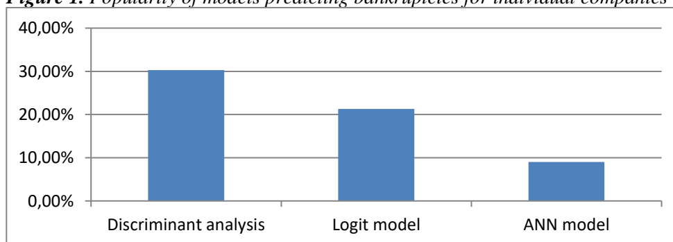
Figure 1. Popularity of models predicting bankruptcies for individual companies
