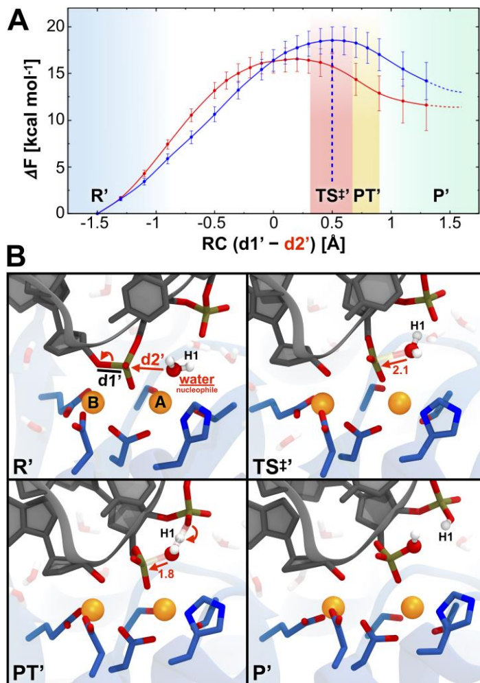
Figure 4. Alternative phosphate-mediated reaction pathway. (A) Free energy profile ( \Delta F^\ddagger , in \text{kcal mol}^{-1} ) for the phosphate-mediated dissociative mechanism (blue line), highlighting regions corresponding to the reactant ( R' ), transition state ( TS^\ddagger' ), proton transfer ( PT' ) and products ( P' ). The free energy profile for the associative pathway activated by H983 is also shown (red line). (B) Snapshots of the R' , TS^\ddagger' , PT' and P' states, as from the dissociative pathway.
