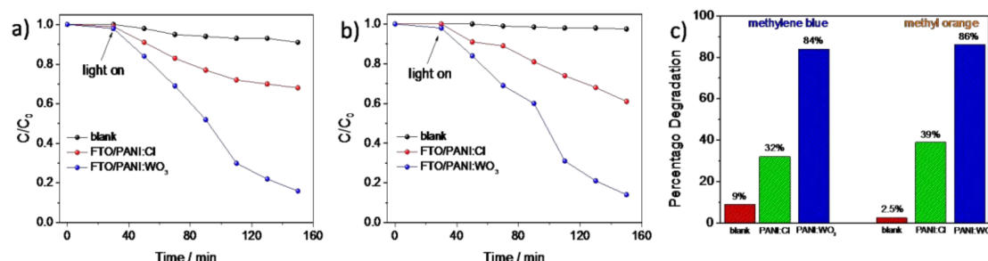
Figure 9. Comparison of the photocatalytic degradation of (a) MB and (b) MO in the presence of PANI/Cl and PANI/ \text{WO}_3 composite photocatalysts under sunlight irradiation and (c) diagram showing the results of photodegradation.
