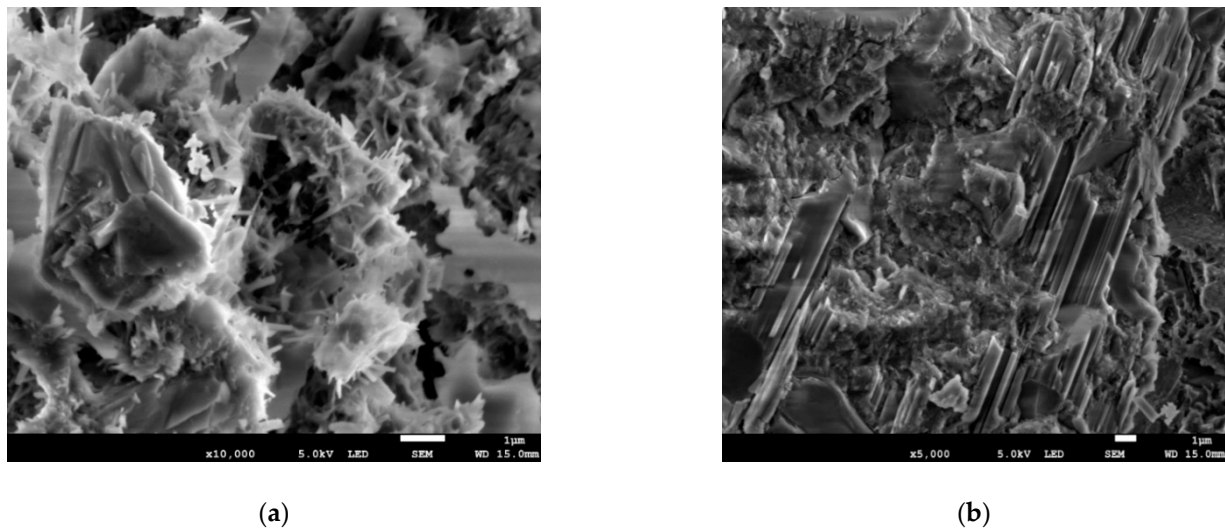
Figure 6. SEM images of the samples taken from center layer of the concrete structure: (a) ×10,000; (b) ×5000.
