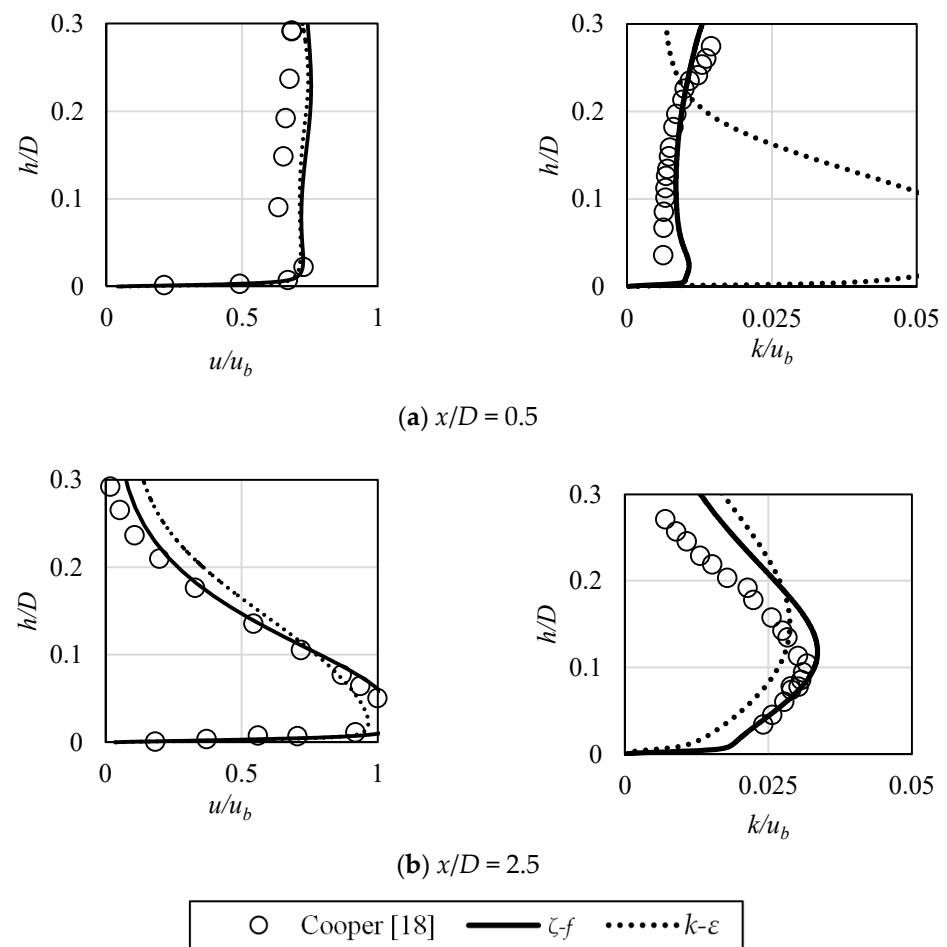
Figure 3. Numerical model validation. Reference experimental data [18] versus k-\epsilon and \zeta-f models results. Velocity profiles (left side) and turbulence kinetic energy profiles (right side) for indicated values of non-dimensional distance x/D from stagnation point.
