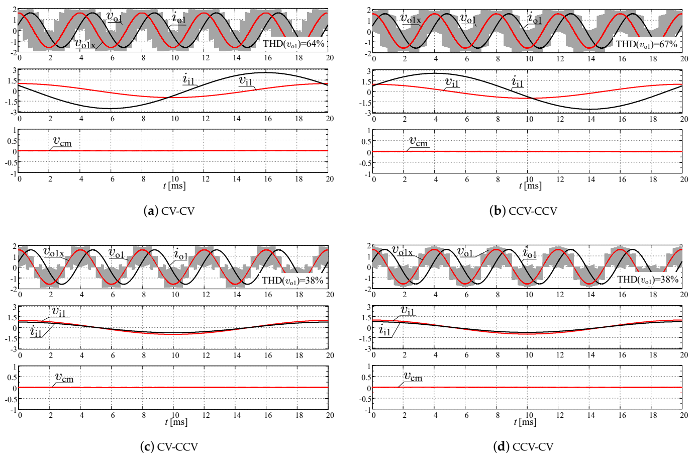
Figure 10. Simulation of the PWM variant 1 for DSM-CMC5 × 5 and four modulation schemes—RL load case.
