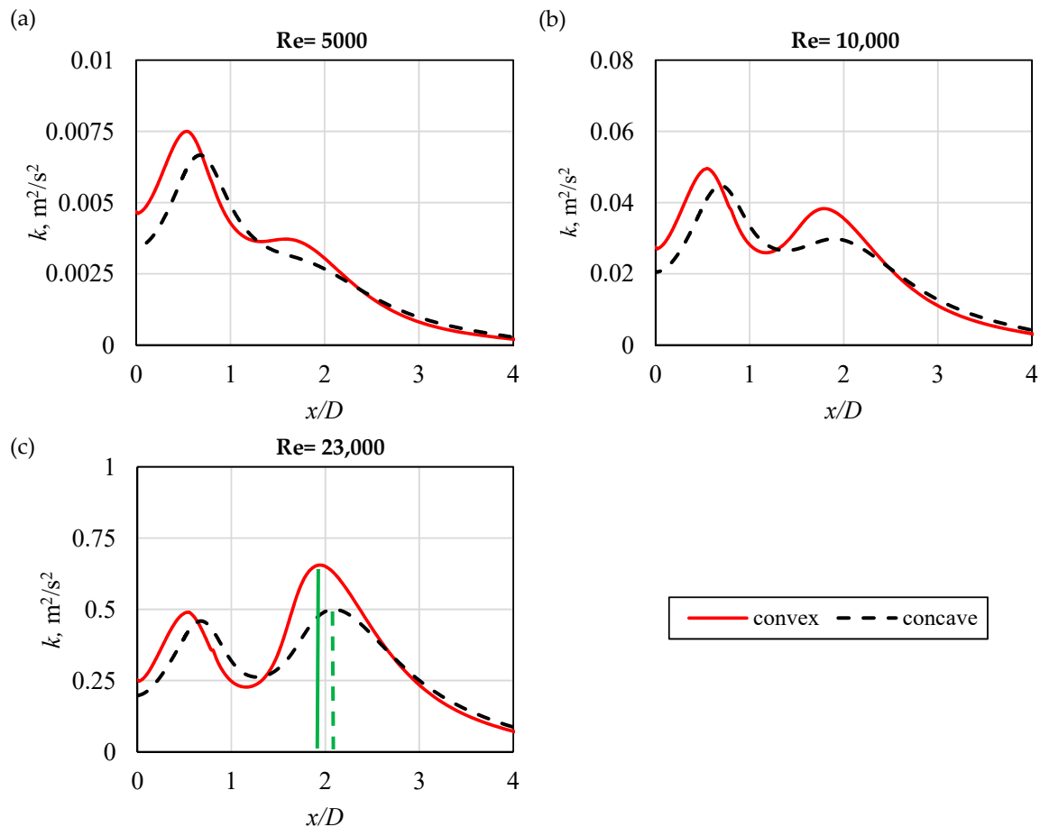
Figure 14. Local values of turbulence kinetic energy, extracted from the first mesh nodes along the impinging wall. H/D = 2 and R/D = 4 . (a) \text{Re} = 5000 , (b) \text{Re} = 10,000 and (c) \text{Re} = 23,000 . Green lines indicate the second maximum of Nusselt number for the same case.
