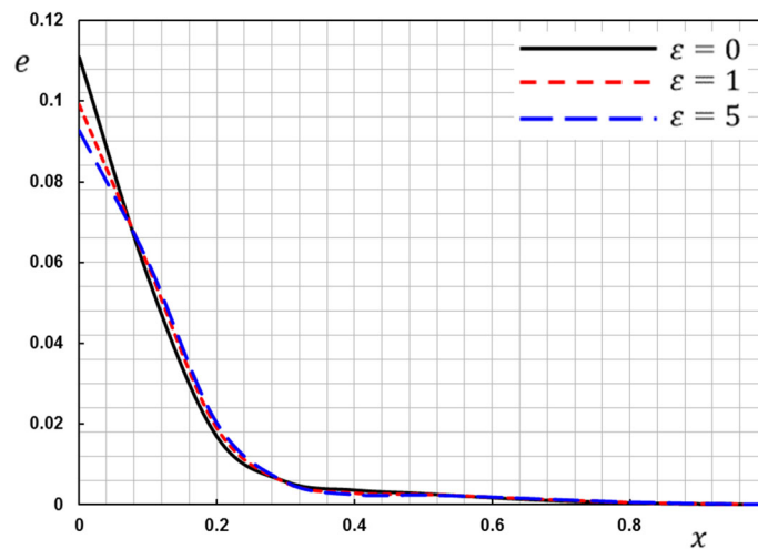
Fig. 13 The strain e under the influence of applied magnetic field
