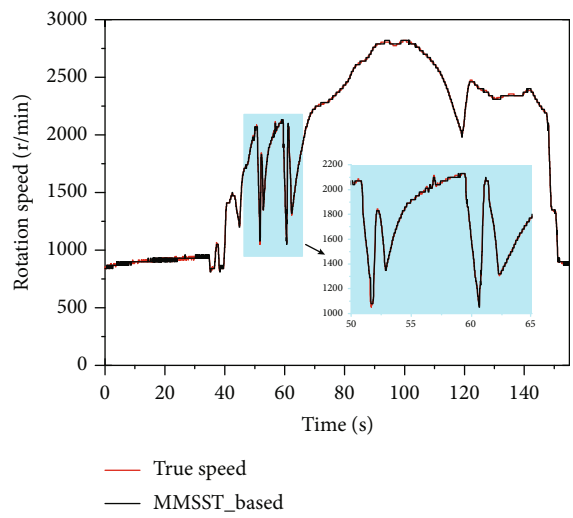
FIGURE 5: The TF results of engine vibration signal and the test results of rotational speed estimation for the applied methods: (a) SST and (b) SST-based estimation result, (c) MSST and (d) MSST-based estimation result, and (e) MMSST and (f) MMSST-based estimation result.
