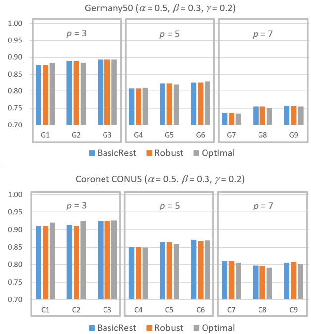
FIGURE 12. Connectivity-based resilience, using WS1, of all Germany50 and Coronet CONUS instances to RAs against p = C - 1 nodes.
