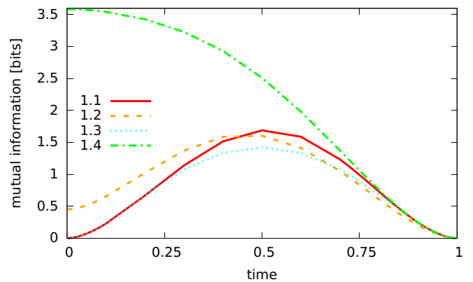
FIG. 8. Plot of I_{\text{mean}}^{(E_1)} (the mean mutual information seen from the reference frame of the first environment, E_1 ) for Cases 1.1, 1.2, 1.3, and 1.4. In Case 1.5 the function is constant and equal to 0. This shows the cases when I_{\text{mean}}^{(E_1)}(t = 1) = 0 . The plot for Case 1.1 is identical for Cases 2.1 and 3.1. (Cases are given in Table II.) When the mutual information is low, the environments have strong independence.
