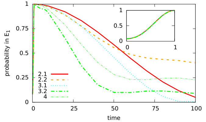
FIG. 7. Probabilities p_0^{(E_1)} for cases from the groups 2, 3, and 4 in the reference frame of E_1 , which have various interactions in addition to central measurement Hamiltonian. Inset: Probabilities during time [0,1] where the measurement-like Hamiltonian dominates. (Cases given are in Table II.)
