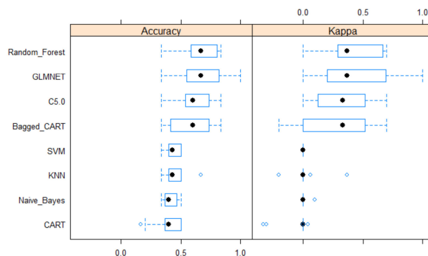
FIGURE 7. Results of validation using leave one out cross validation algorithm.
