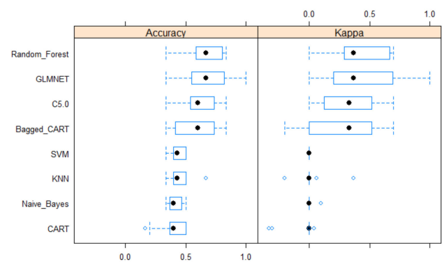
FIGURE 6. Results of validation using repeated k-fold cross-validation algorithm.
