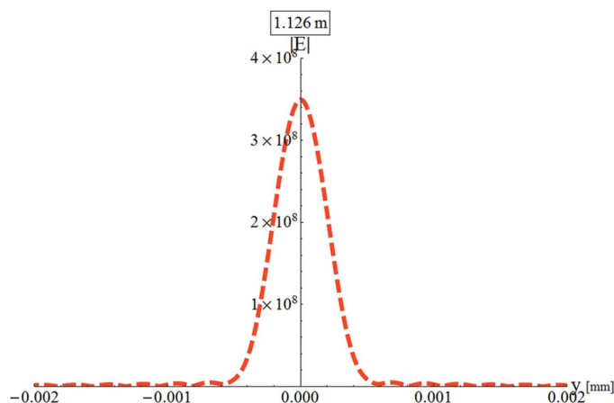
Figure 6 Focus spot obtained with 10 kinoform lenses (blue line) and 10 ideal lenses (red dashed line).
