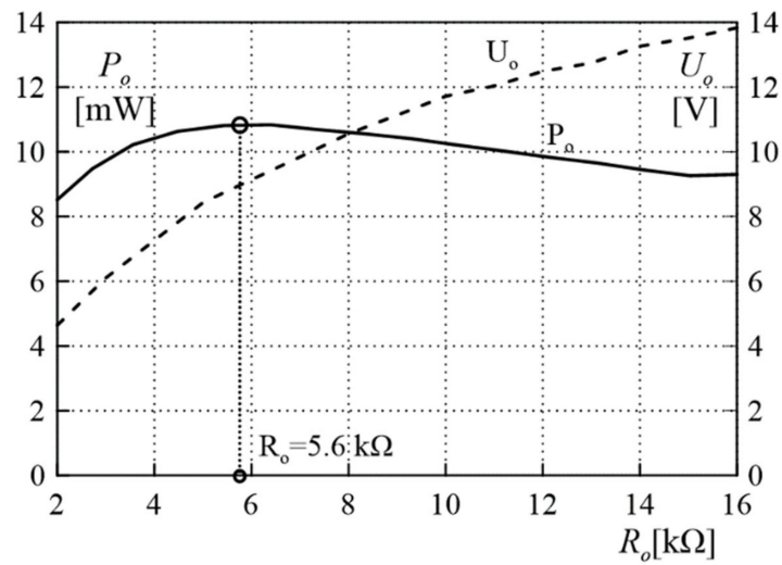
Figure 18. The output power P_o and voltage U_o generated by proposed EH system as a function of load resistance for the first resonance frequency ( f_0 = 332 MHz).
