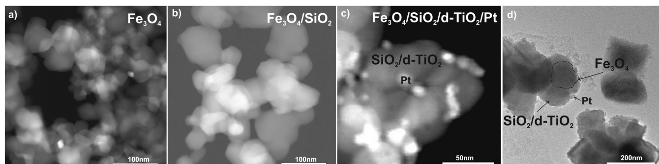
Fig. 2. TEM images presenting all stages of building the core-shell defective \text{Fe}_3\text{O}_4@\text{SiO}_2/\text{d-TiO}_2/\text{Pt} magnetic nanocomposite: \text{Fe}_3\text{O}_4 (a), \text{Fe}_3\text{O}_4@\text{SiO}_2 (b), and final composite (c-d).
