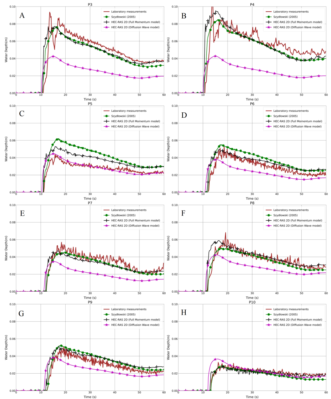
Figure 6 (A-H) Laboratory measurements compared to both the Full Momentum model and the Diffusion Wave model, as well as to the solution by Szydlowski (2005) , for the modified DEM with the aligned building layout (1a-BB). Full-size DOI: 10.7717/peerj.11667/fig-6
