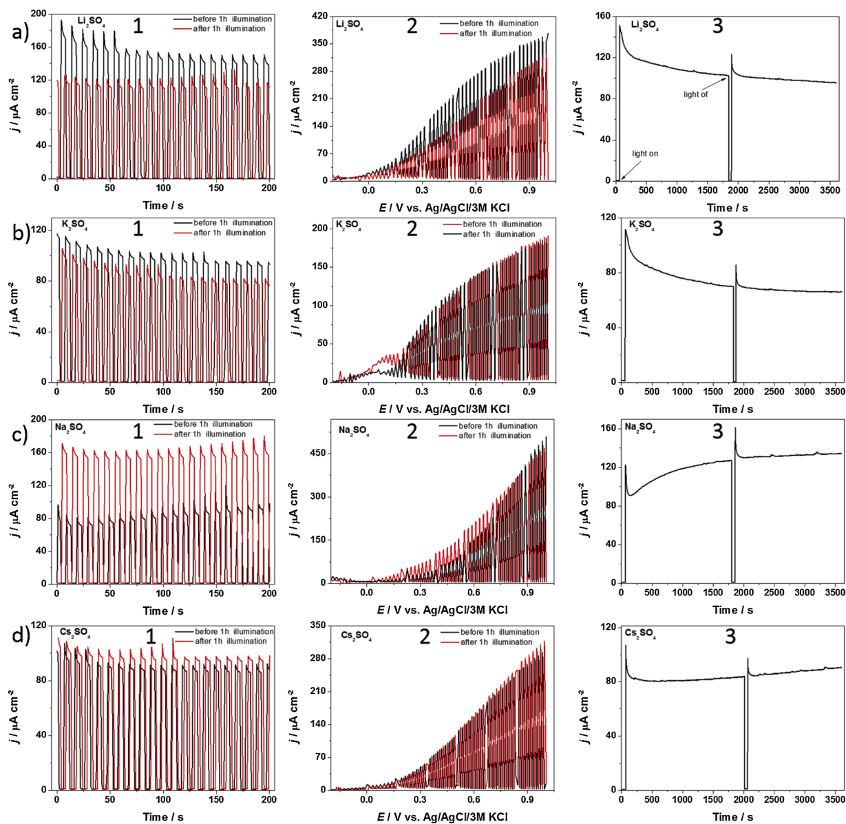
Fig. 11. The comparison of CA, LV curves of exfoliated WO 3 before and after illumination and the long-term chronoamperometry test ( E = 0.5 V vs. Ag/AgCl (3 M KCl)) recorded during illumination of electrode. Measurements performed in various electrolytes a) Li 2 SO 4 , b) K 2 SO 4 , c) Na 2 SO 4 and d) Cs 2 SO 4 .
