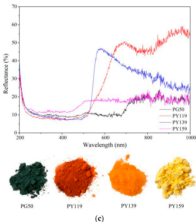
Figure 4. Aging factor of EN as a function of aging time for EN samples containing 1 phr (a) and 3 phr (b) of pigment; reflectance spectra of the pigment powders (c).
