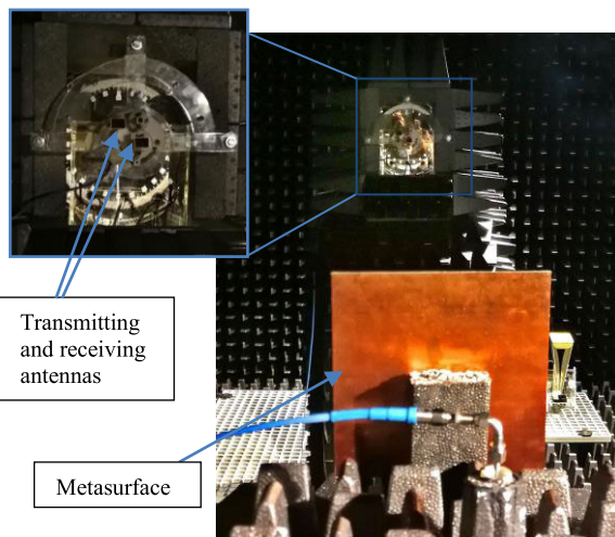
FIGURE 15. Measurement setup at Reykjavik University.
