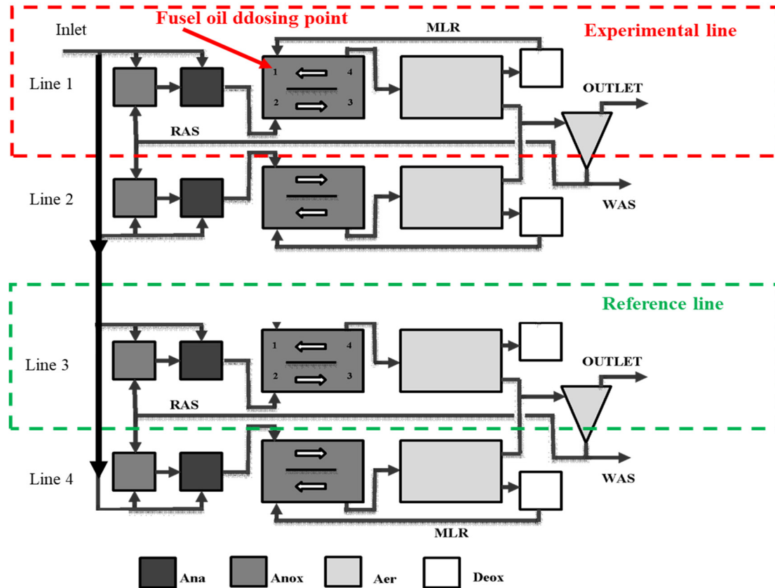
Figure 1. Layout of the full-scale JHB systems for investigating the acclimation of biomass to fusel oil at Poznan WWTP. Abbreviations: RAS—recalcitrated activated sludge, MLR—mixed liquor recirculation, WAS—waste activated sludge. Reactors: Ana—anaerobic, Anox—anoxic, Aer—aerobic, Deox—deoxidation of the MLR.
