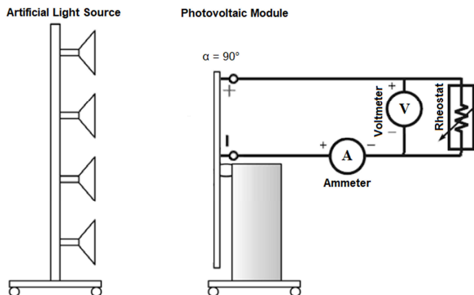
Fig. 3. Scheme of the measuring unit in the laboratory
