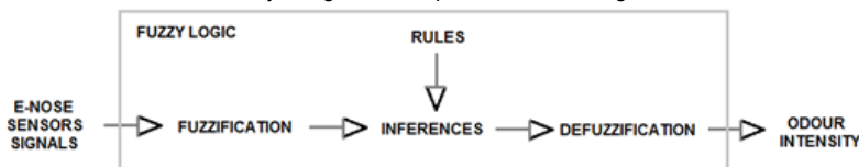
Figure 2: Scheme of using electronic nose combined with fuzzy logic to estimate the odour intensity
