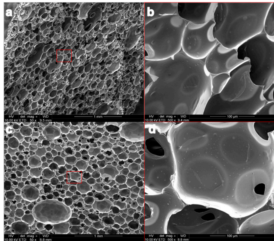
Figure 3. SEM images of PUR ((a,b), where (b) shows the fragment from the red selection of image (a)) and PUR+Ch2 foam ((c,d), where (d) shows the fragment from the red selection of image (c)).
