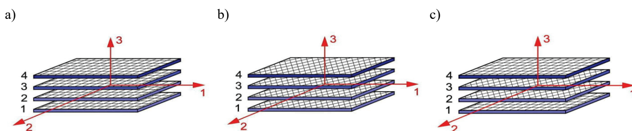
Fig. 3. Example sequence of the plies in specimen: a) [BAT 4 ], b) [GBX 4 ], c) [BAT,GBX 2 ,BAT]
